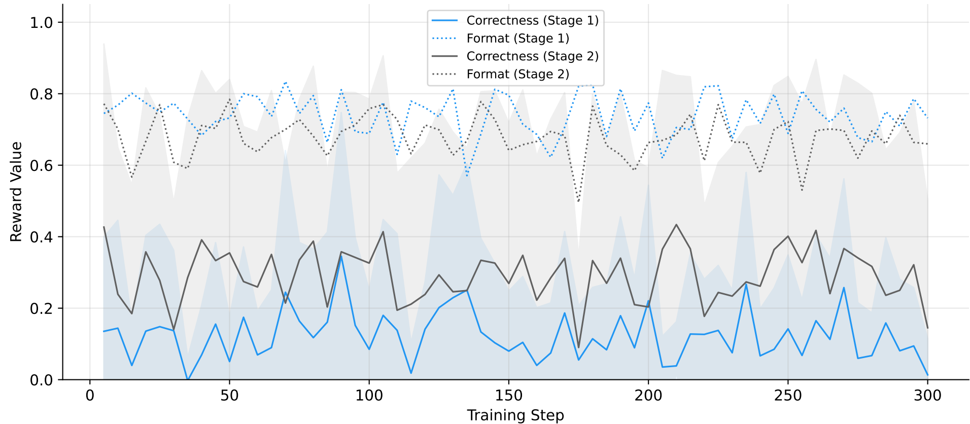
GSPO: Reward Decomposition (GDPO Decoupled)
